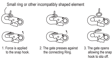
Fig. 3 - Inappropriate Connections
