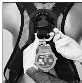
Push the pin inside the grooves of the connector to ensure locking.
