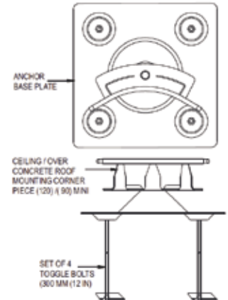
ANCHOR POST (CORNER) WITH SET OF 4 NOS TOGGLE ANCHOR
