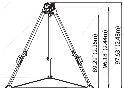
Maximum Height in Open Condition
