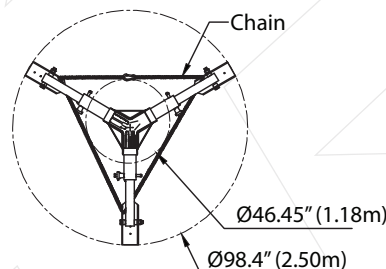
Foot Print Diameter at Minimum Height
