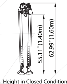
Height in Closed Condition
