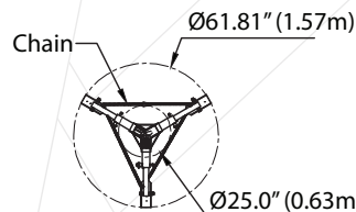
Foot Print Diameter at Minimum Height
