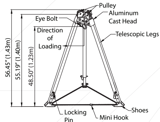
Height in Closed Condition
