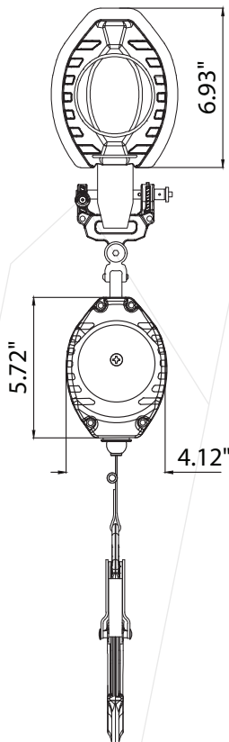
FRONT VIEW
