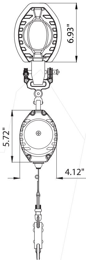
FRONT VIEW
