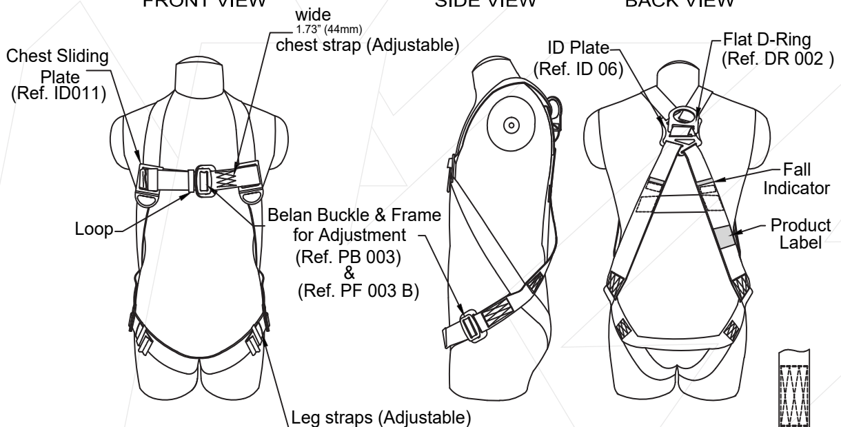
STITCHING DESIGN
