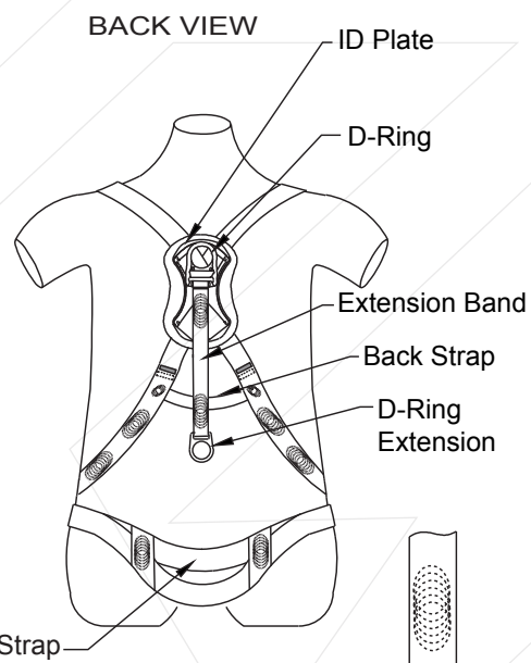
STITCHING DESIGN
