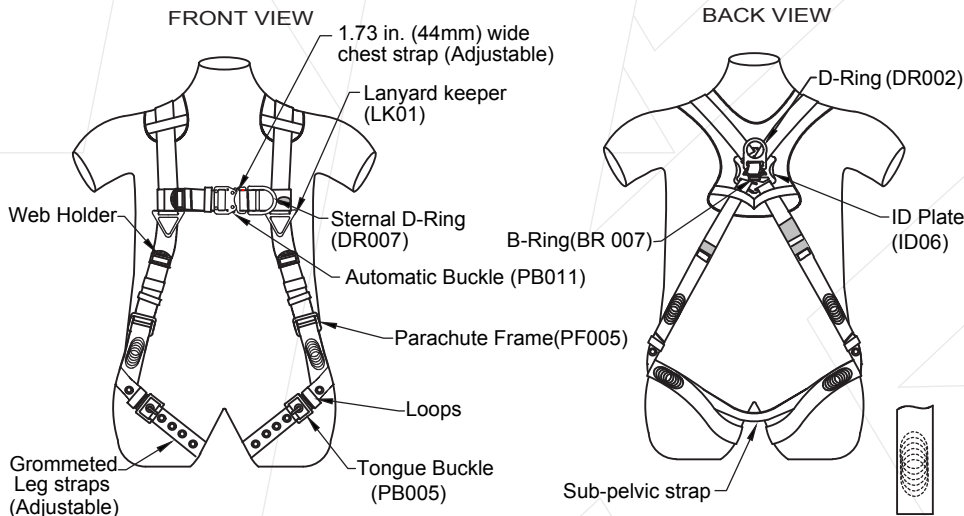
STITCHING DESIGN
