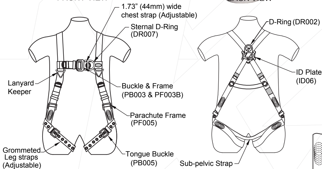
STITCHING DESIGN
