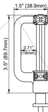
OPEN CONDITION
