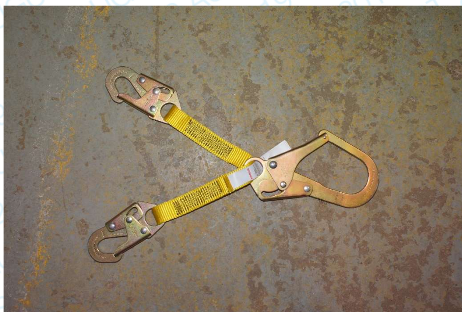
Figure 1 – Lanyard/positioning lanyard described as "FAP 30698"
