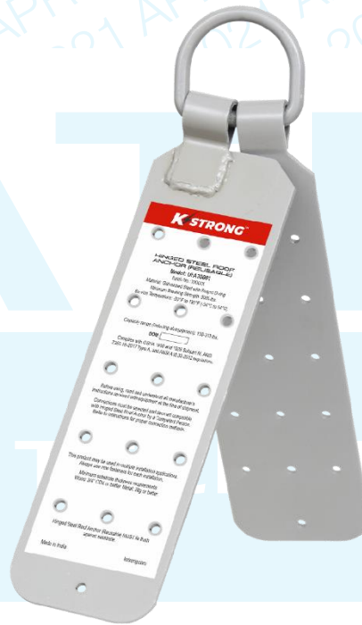
Figure 1 – Anchorage connector described as “UFA30001” (photo supplied by manufacturer)
