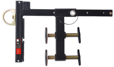
PARAPET ANCHOR 285MM WITH EXTENDED MOVABLE ARM 23KN (AFA930101)
