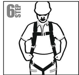
Step 6 : Tighten the leg straps by pulling the free ends of The straps until the harness fits perfectly to the body as shown in Step 6.
