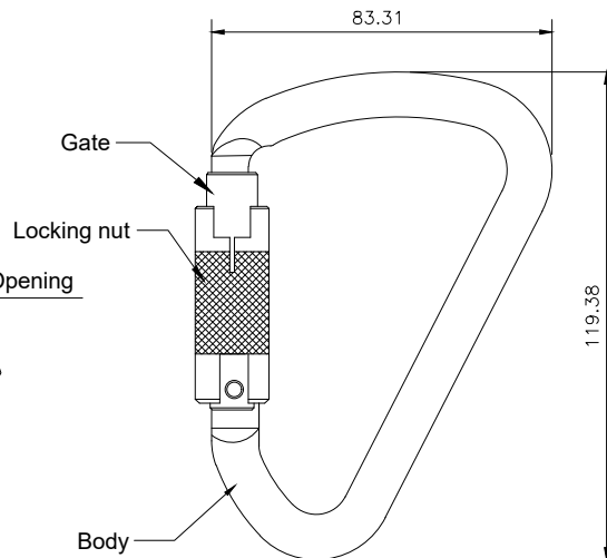
CLOSED CONDITION
