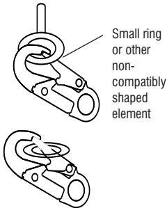
1. Force is applied to the snap hook.
