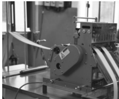
Webbing Cutting Machine
