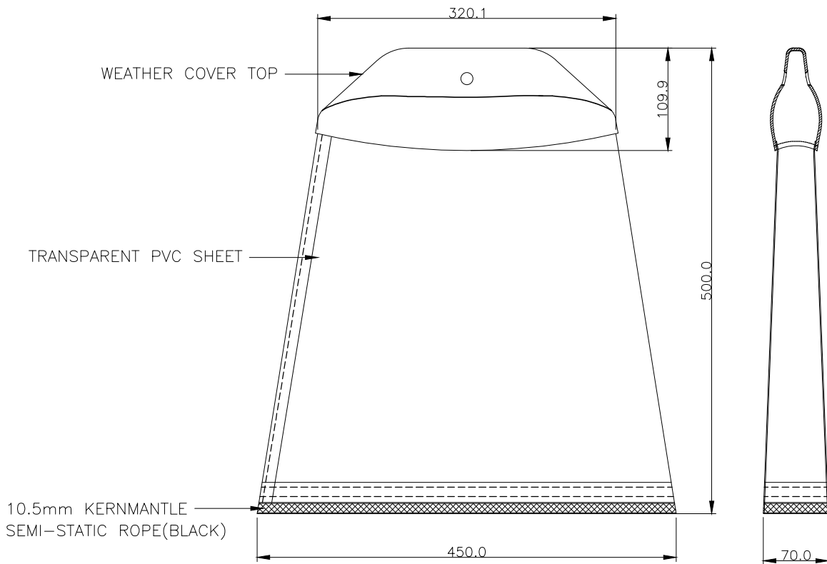
SIDE VIEW
